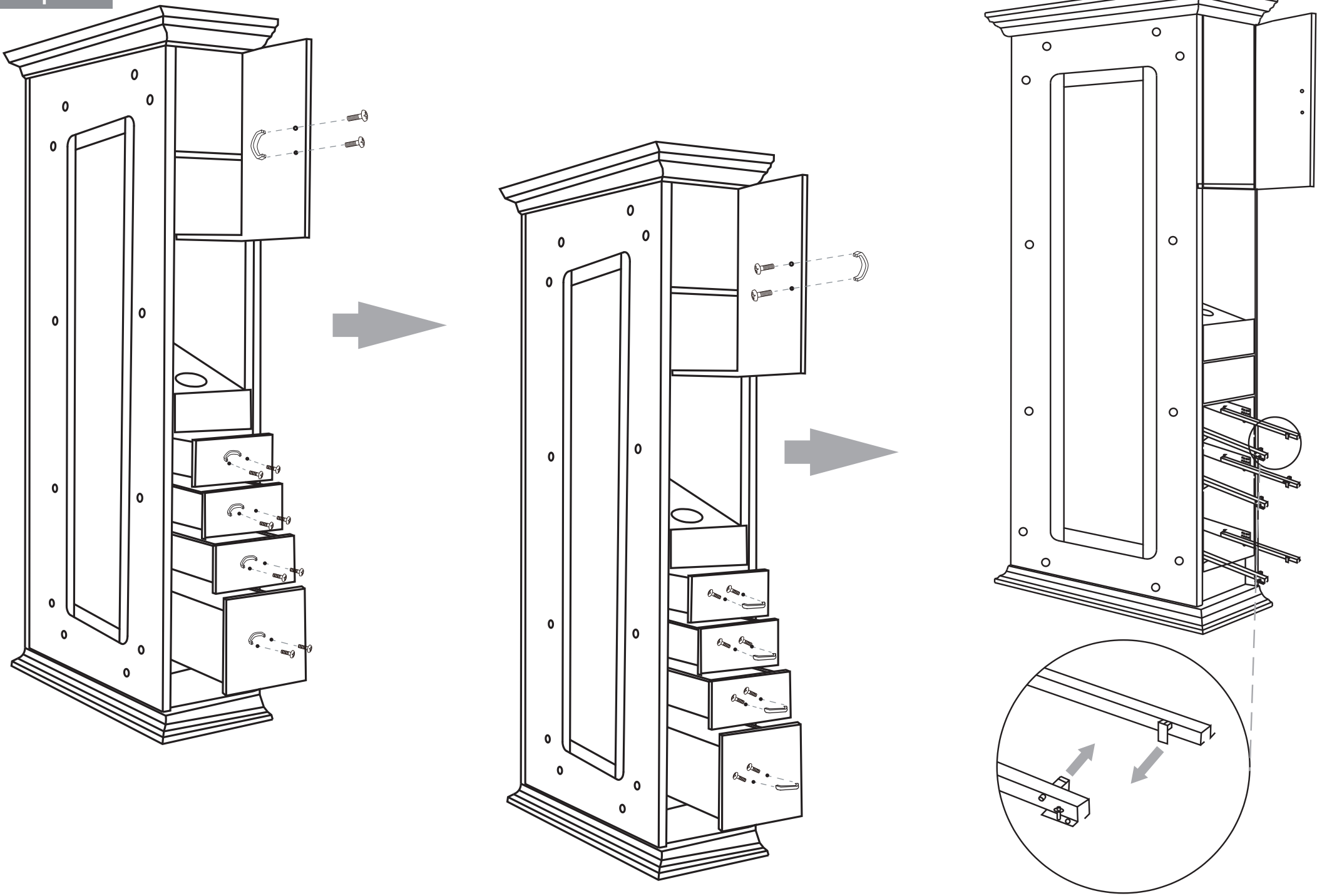
Remove all drawers for installation of the mirror
